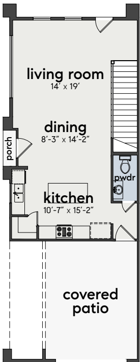
First Floor
