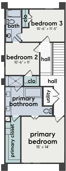
Second Floor
