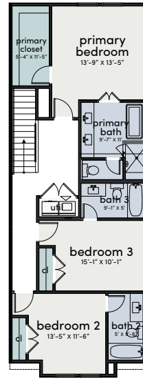
SECOND FLOOR
