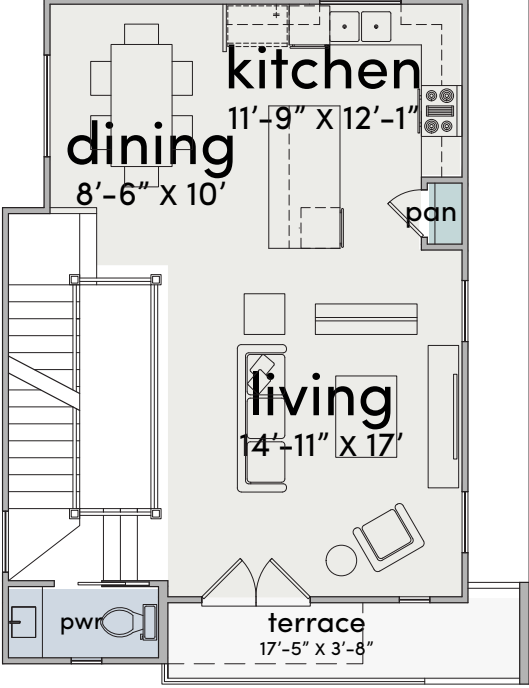
SECOND FLOOR
