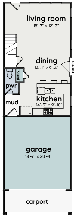
First Floor
