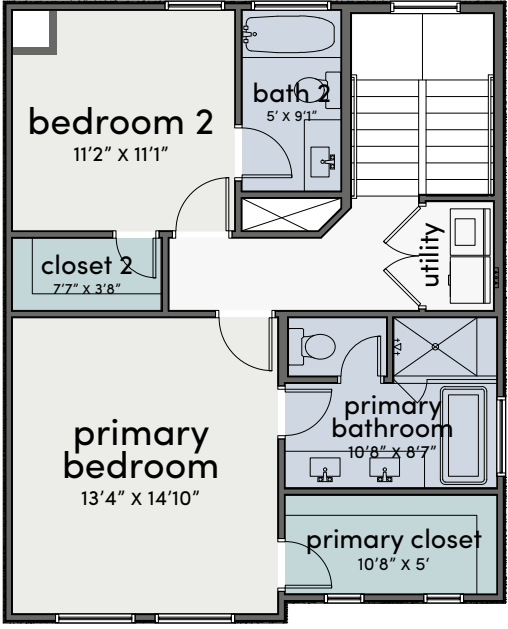
THIRD FLOOR
