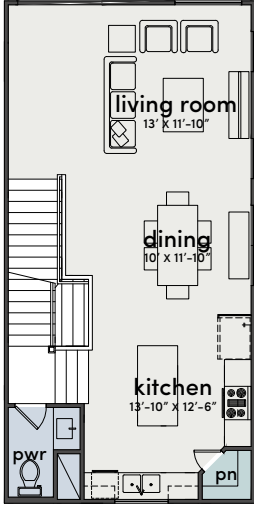
PLAN A 3 BEDS | 3.5 BATHS | 1,757 SQFT
