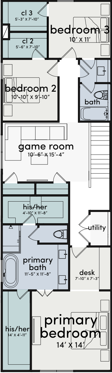
SECOND FLOOR
