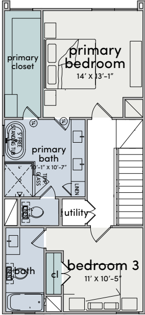
THIRD FLOOR
