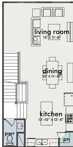
PLAN A 3 BEDS | 3.5 BATHS | 1,755 SQFT
