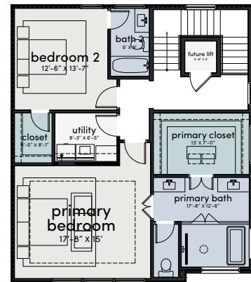
THIRD FLOOR
