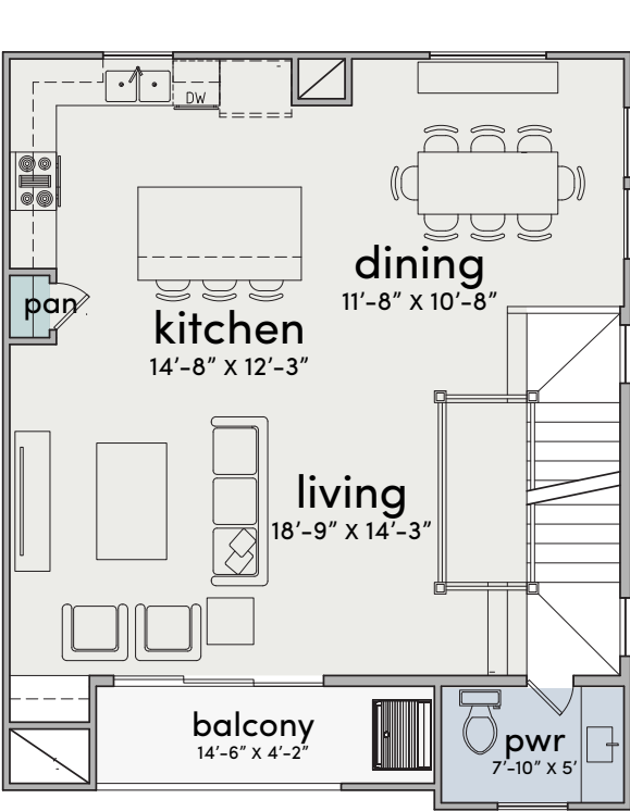
SECOND FLOOR
